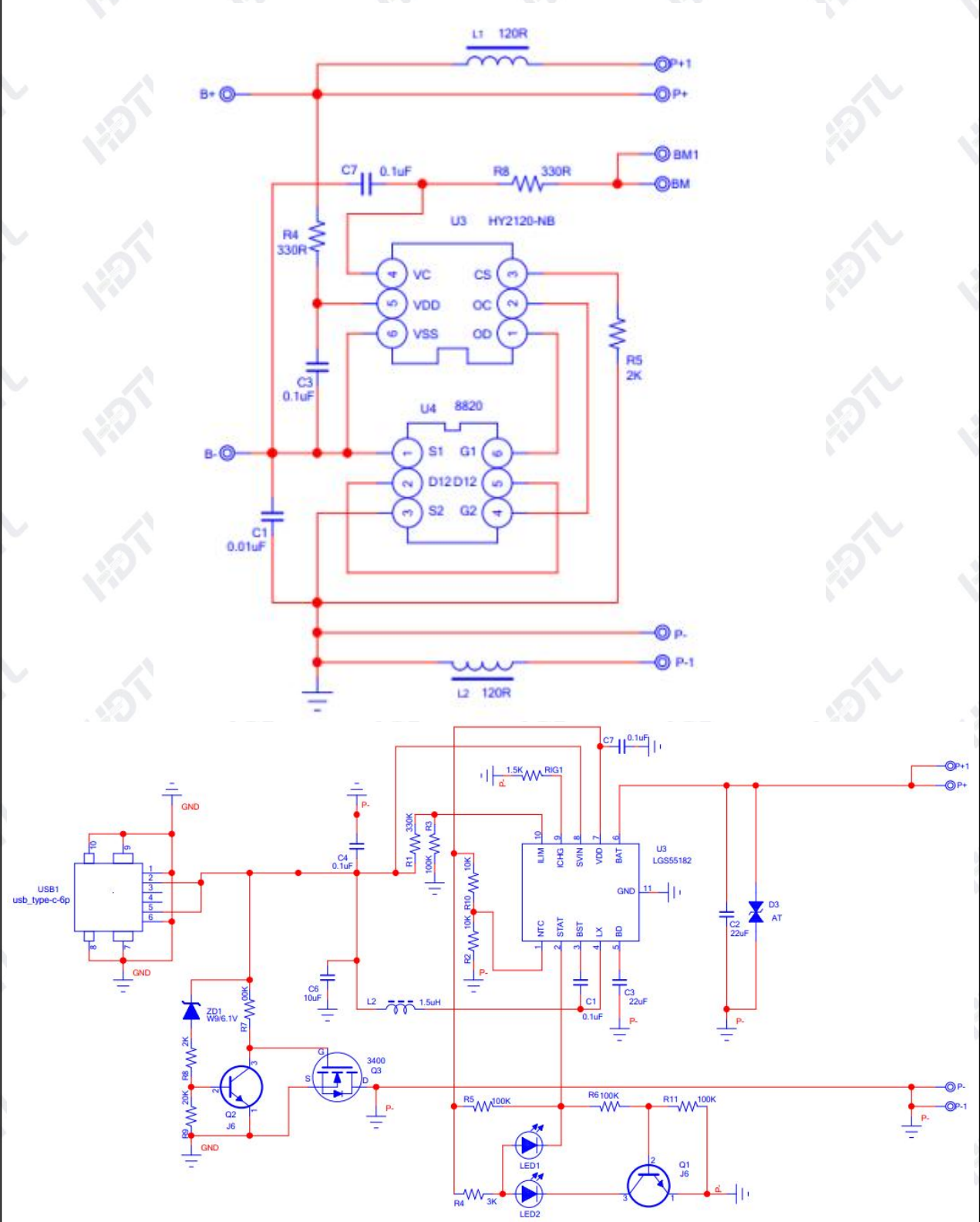
Circuit diagram:
