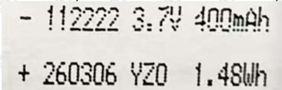
Label of battery
