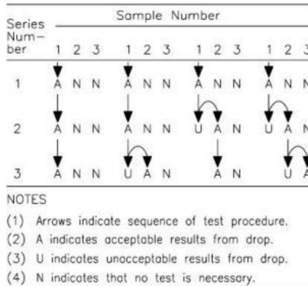
Figure 16.2.3.1 Procedure for impact test (See Clause 16.2.3.2.)
