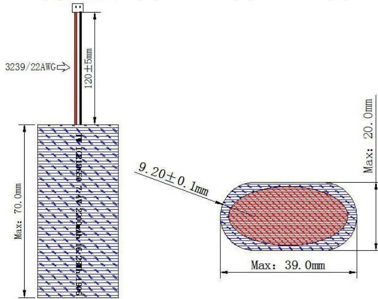
Battery
