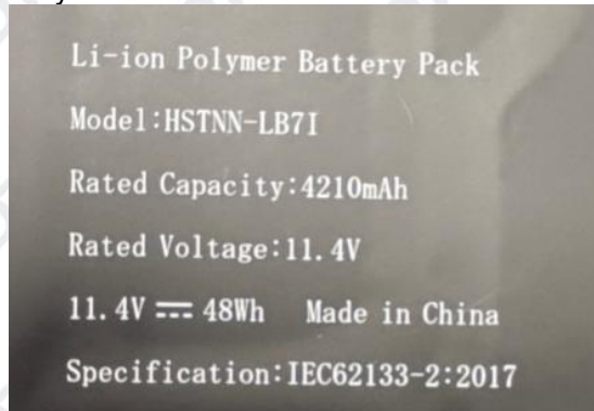
Label of battery
