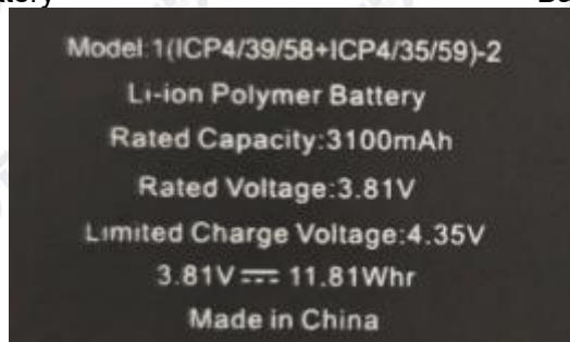
Label of battery
